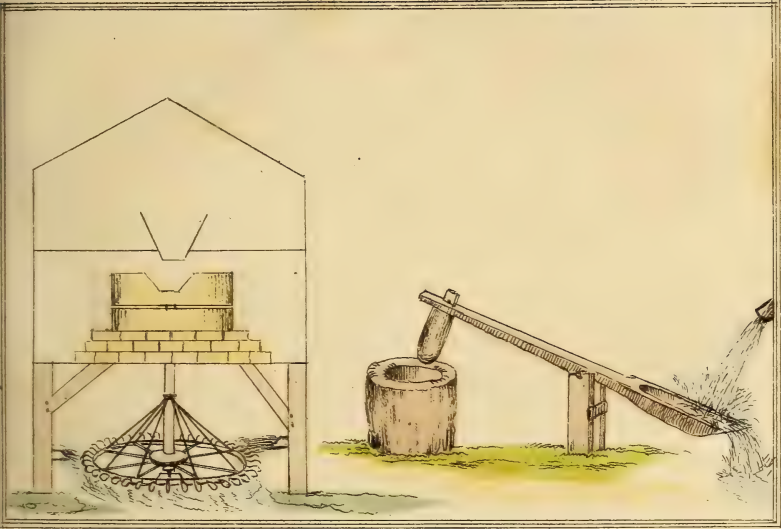
HORIZONTAL CORN MILL.
