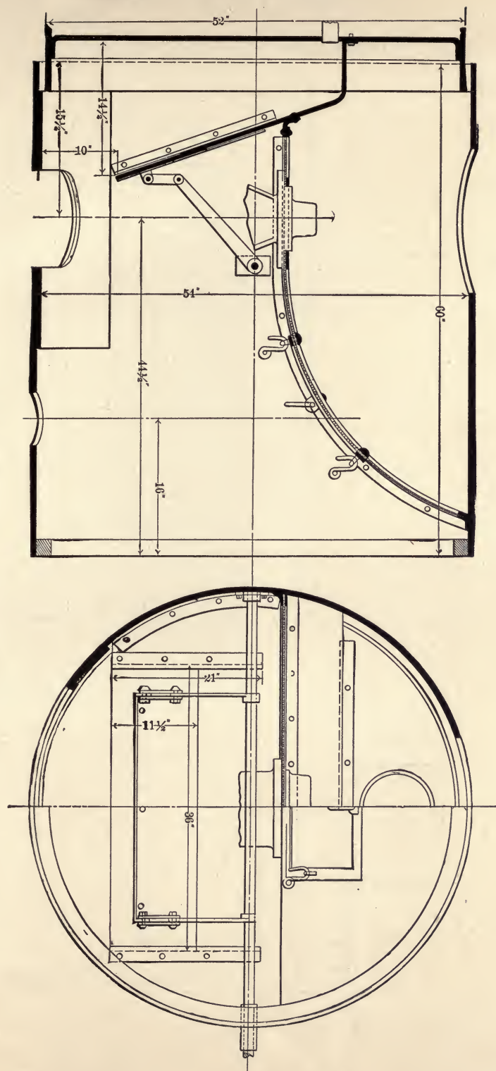
Fig. 34.—Netting and Deflector-plate.
