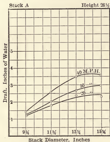
FIG. 125.—Straight Stack, Nozzle No. 2.
