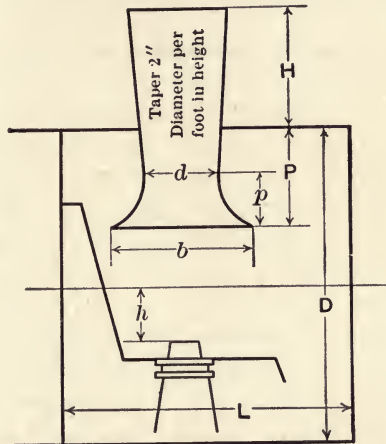
BEST ARRANGEMENT OF FRONT END.
