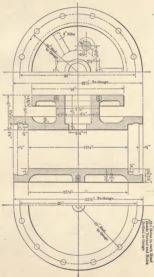
FIG. 38.—Cylinder-heads.
