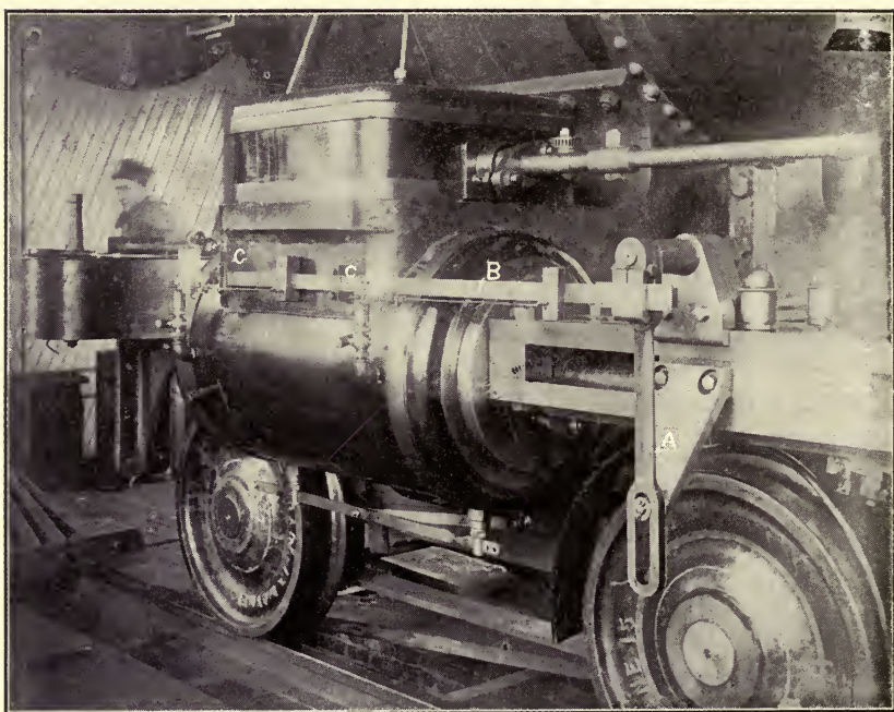
FIG. 153.—Indicator Rigging.
