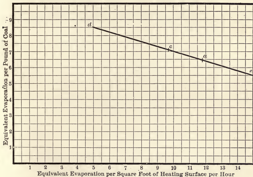
FIG. 215.—Evaporative Performance.
