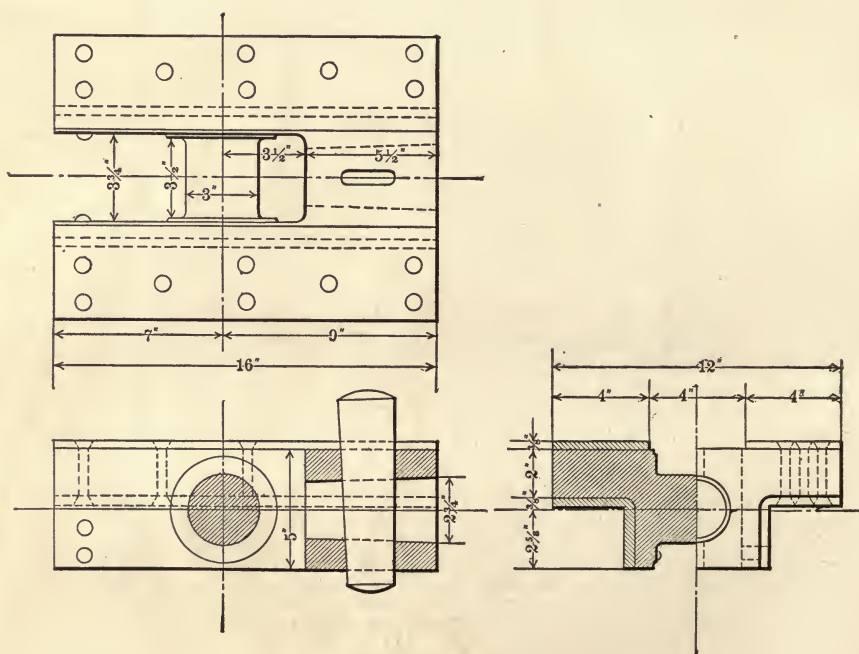
FIG. 40.—Cross-head.
