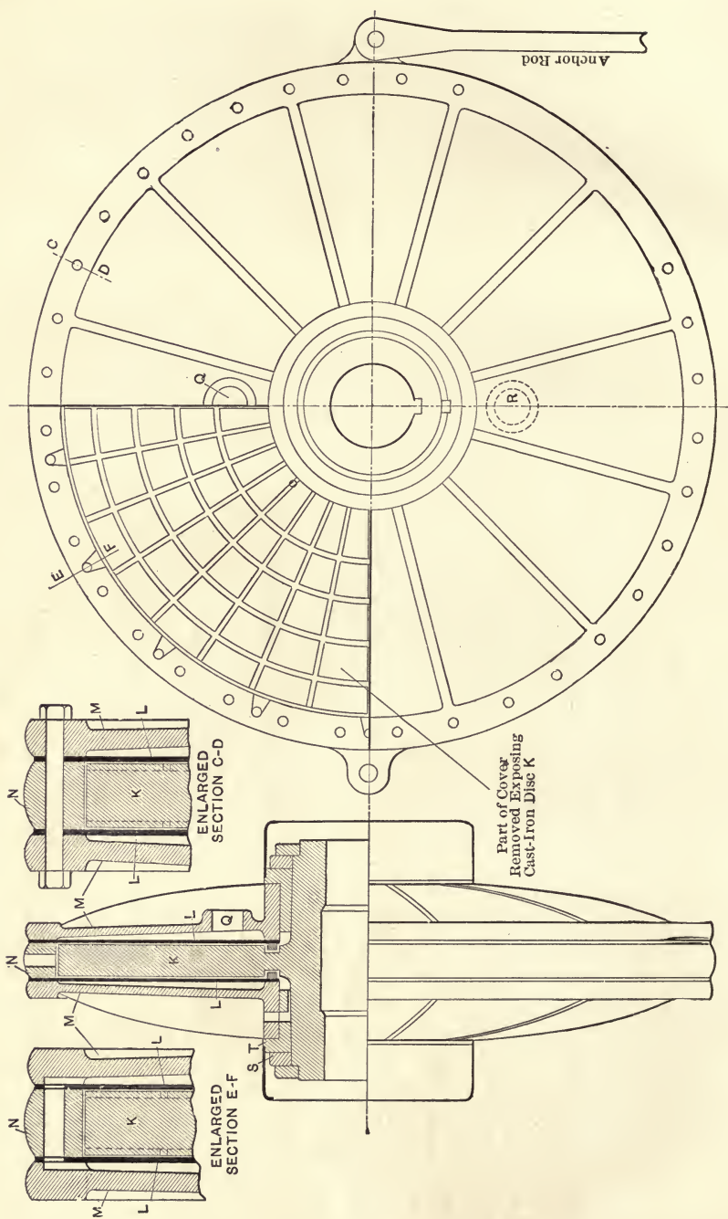
Fig. 10.—Alden Friction-brake.
