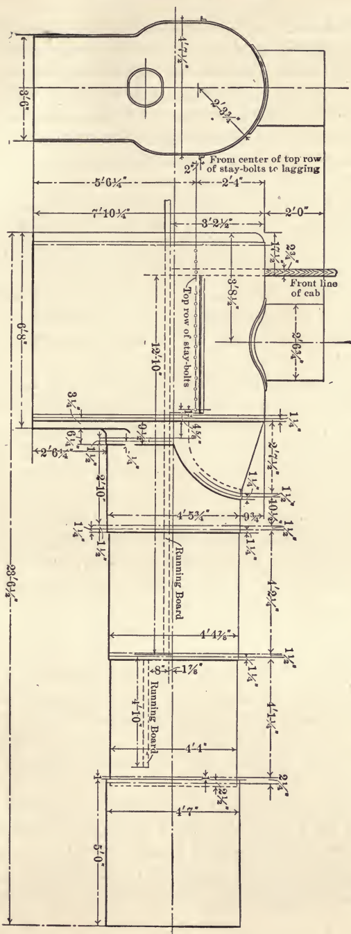
FIG. 101.—Experimental Boiler.
