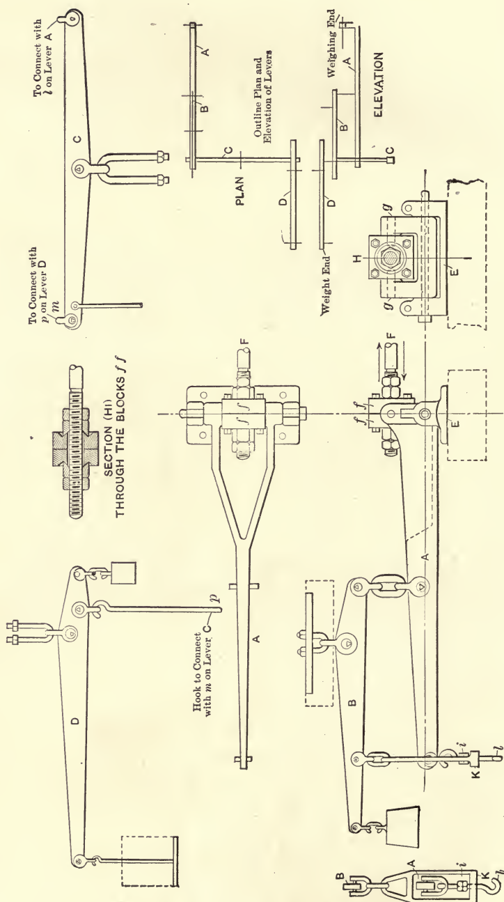
Fig. 13.—Locomotive Dynamometer.
