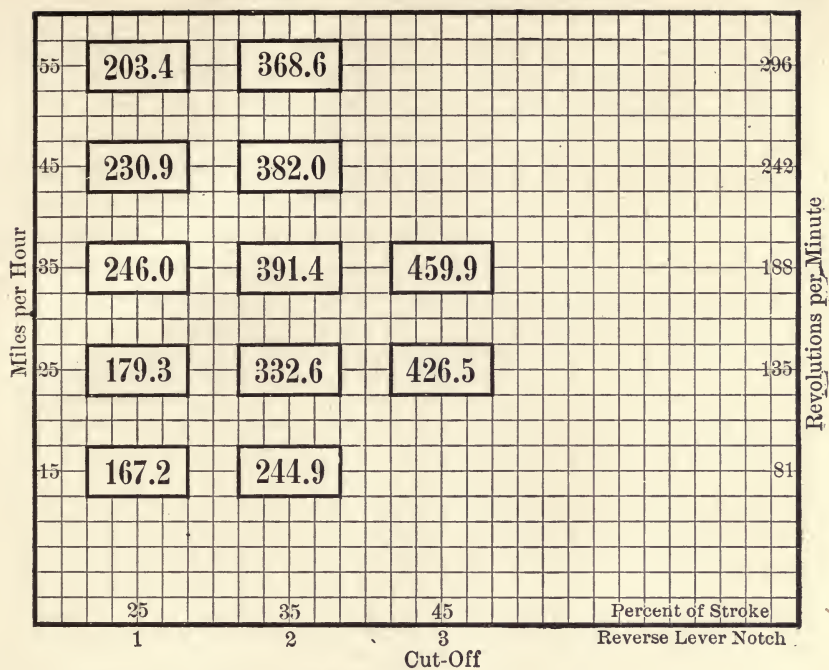
FIG. 74.—Dynamometer Horse-power.
