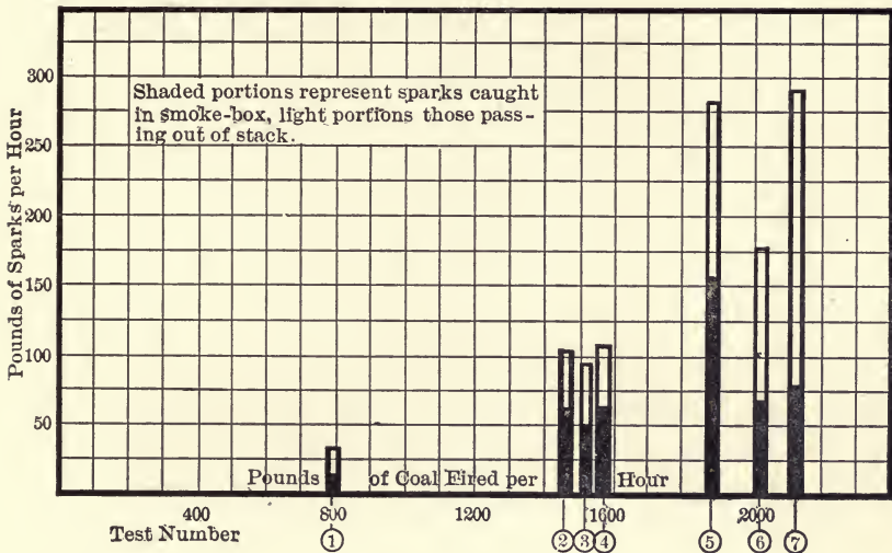
FIG. 94.—Spark Losses.
