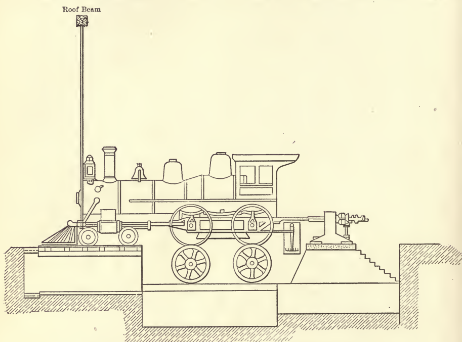
FIG. 206.—Method Used to Determine Position of Engine.
