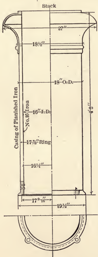
FIG. 30.—Stack.
