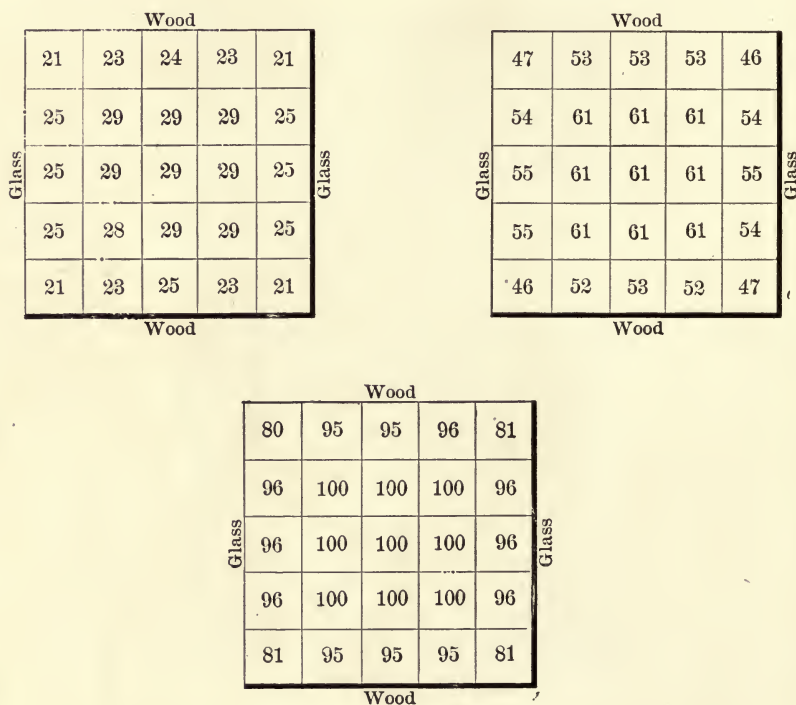
FIG. 220.—Relative Velocities in Different Portions of the Conduit.
