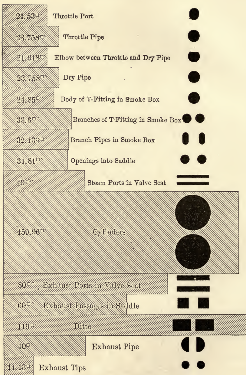
FIG. 54.—Steam-passage Areas.
