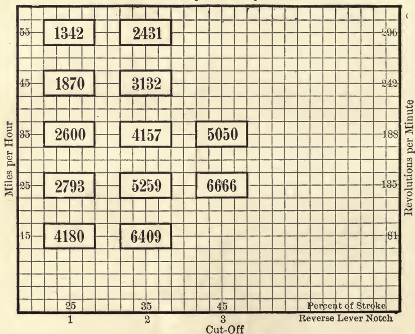
FIG. 73.—Draw-bar Pull.
