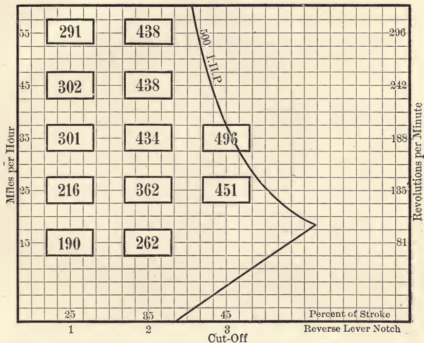
FIG. 64.—Indicated Horse-power.
