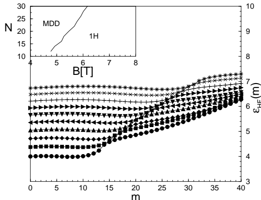
FIG. 1. Hartree-Fock quasi-particle energies \epsilon_{HF}(m) of the MDD state as a function of m for different values of N . \tilde{\gamma} is chosen, for each N , so that the MDD is close to its instability point; \tilde{\gamma} = 0.077, 0.08, 0.082, 0.085, 0.0875, 0.0925, 0.0975, 0.1, 0.108, 0.113 for N = 30, 28, 26, \dots, 14, 12 , respectively. The inset displays the HF phase boundary between the MDD state and one-hole states for a dot with \hbar\Omega = 3\text{meV} . The dimensionless confinement strength parameter \tilde{\gamma} , the field in Tesla B , and the confinement oscillator frequency in meV are related by B[\text{Tesla}] = [0.131(\hbar\Omega[\text{meV}])^2/\tilde{\gamma}]^{2/3} .
